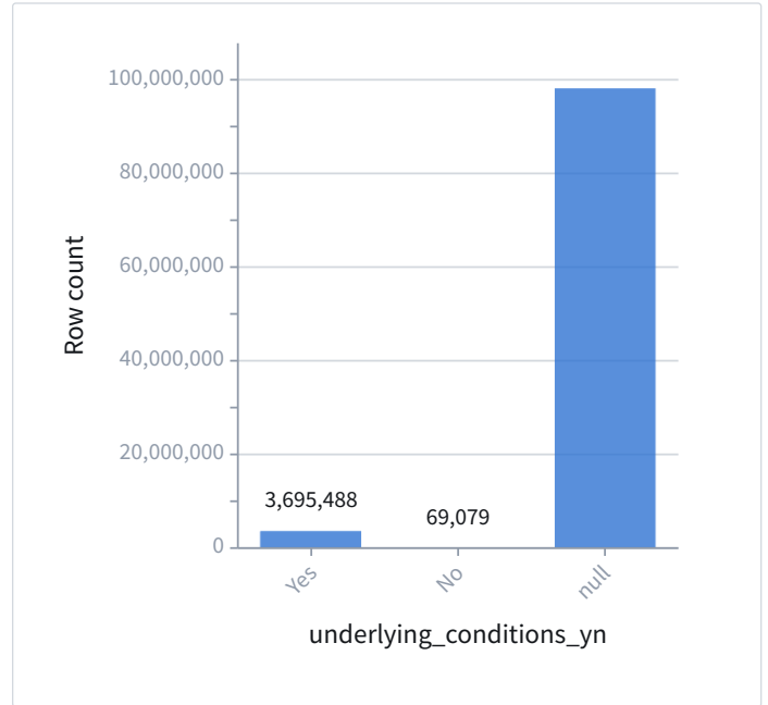
underlying_conditions_yn
